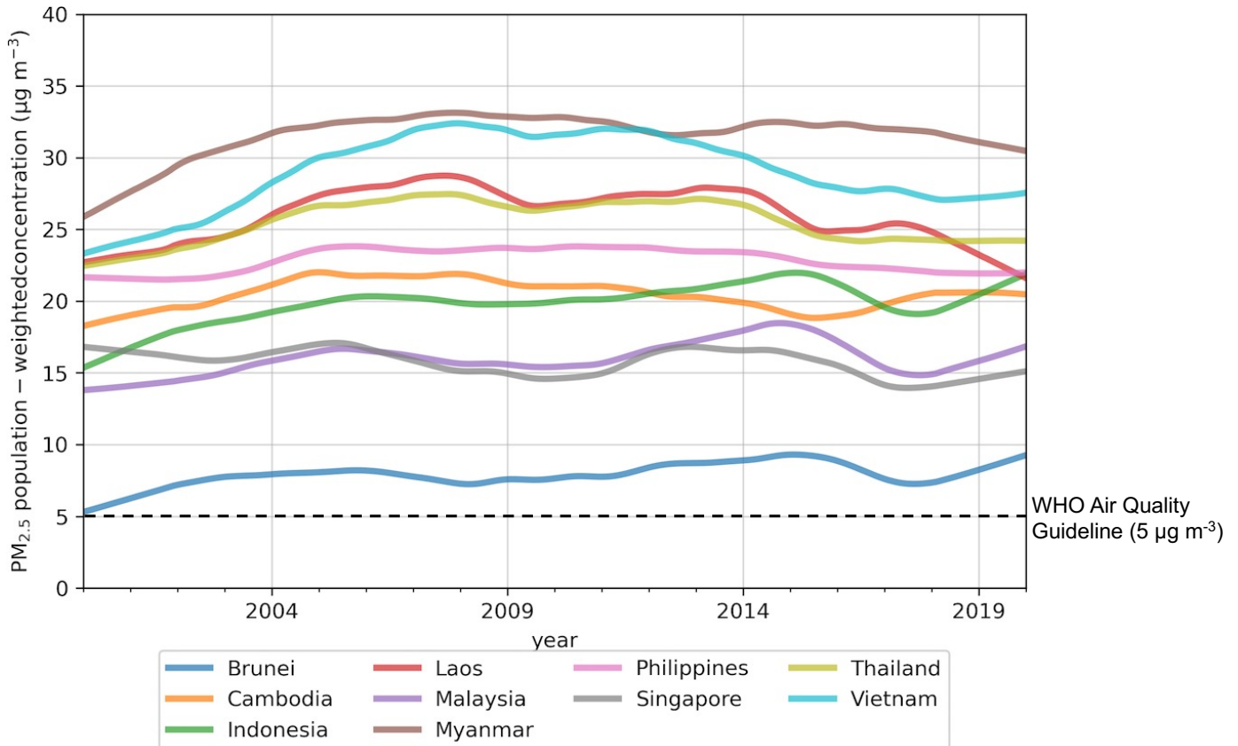
Figure 1. National population-weighted PM 2.5 concentrations for Southeast Asian countries between the years 2000 to 2020. Figure was produced using PM 2.5 data from van Donkelaar et al.[4] and population data from CIESIN[5].
